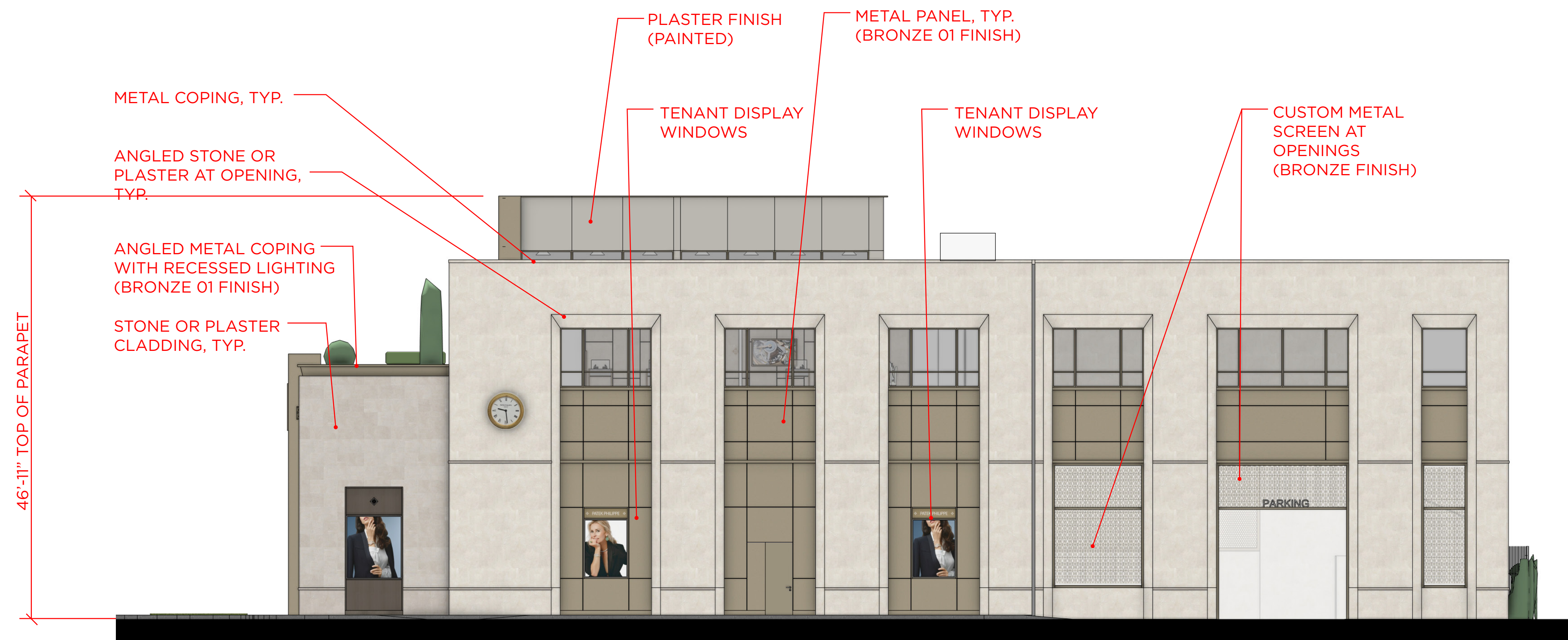
NORTH ELEVATION
