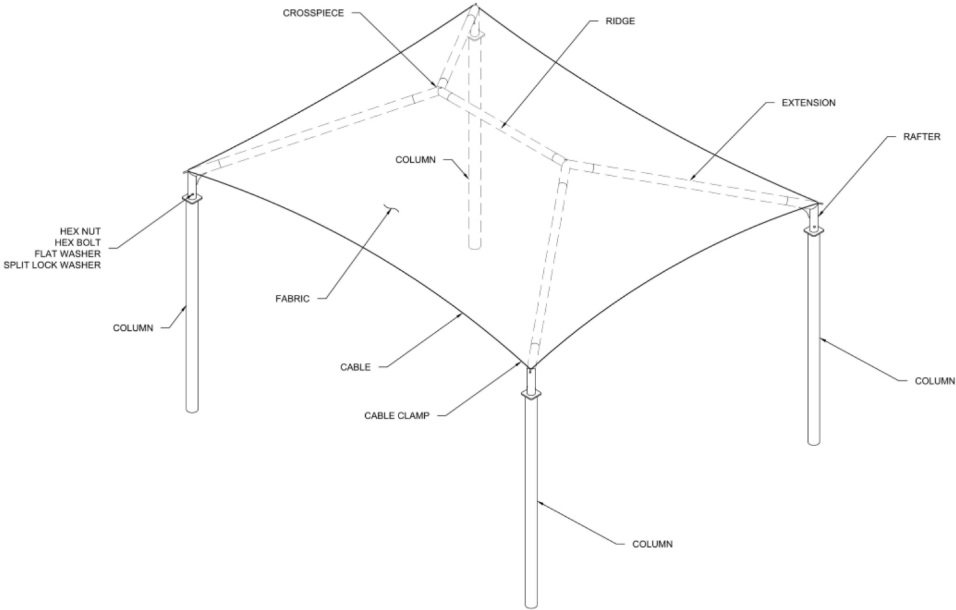
ISOMETRIC VIEW
