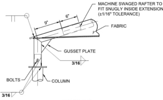
VIEW B-B
