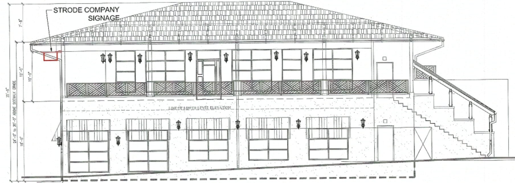
South Elevation
