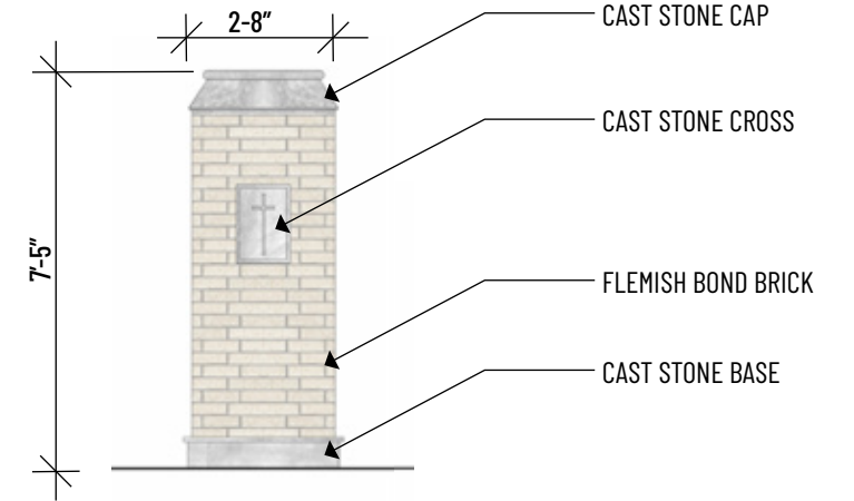
1 NORTH & SOUTH CENTER COLUMBARIUM WALL (LOWER COURT) 1/4" = 1'-0"
