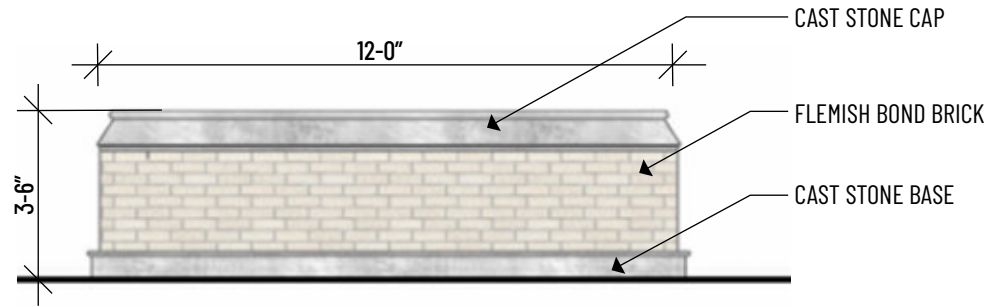
5 EAST SANCTUARY COLUMBARIUM WALL (UPPER COURT) 1/4" = 1'-0"
