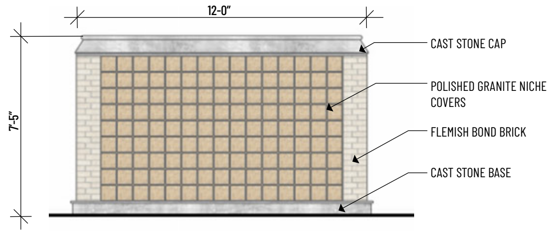
6 EAST SCHOOL COLUMBARIUM WALL (UPPER COURT) 1/4" = 1'-0"
