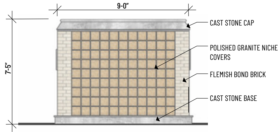
2 WEST CENTER COLUMBARIUM WALL (LOWER COURT) 1/4" = 1'-0"
