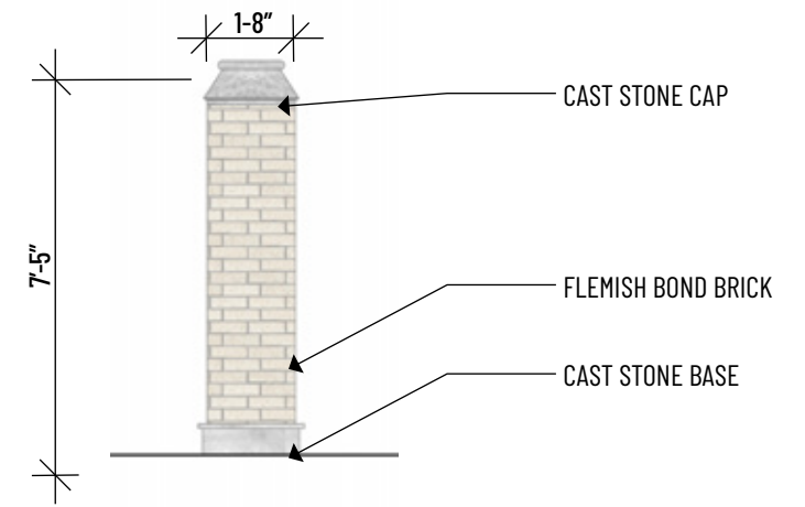
4 NORTH & SOUTH SCHOOL COLUMBARIUM WALL (UPPER COURT) 1/4" = 1'-0"
