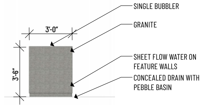
⑥ SOUTH ELEVATION (LOWER COURT) 1/4" = 1'-0"
