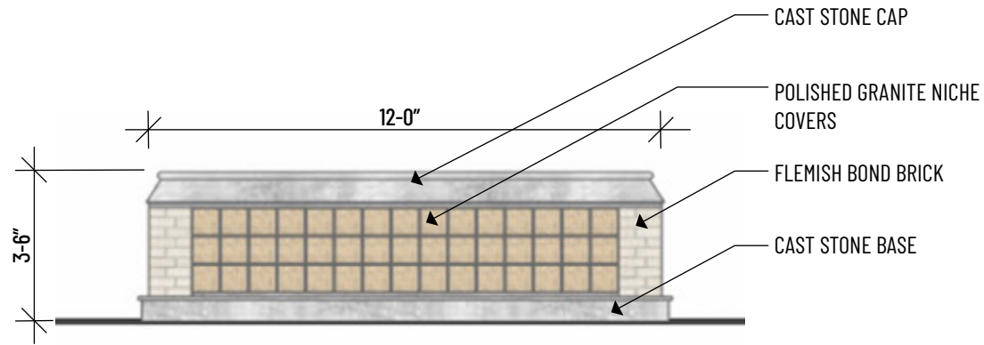
6 WEST SANCTUARY COLUMBARIUM WALL (UPPER COURT) 1/4" = 1'-0"
