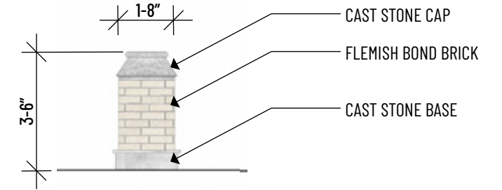
4 NORTH & SOUTH SANCTUARY COLUMBARIUM WALL (UPPER COURT) 1/4" = 1'-0"
