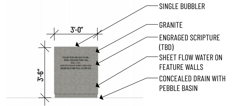
④ NORTH ELEVATION (LOWER COURT) 1/4" = 1'-0"
