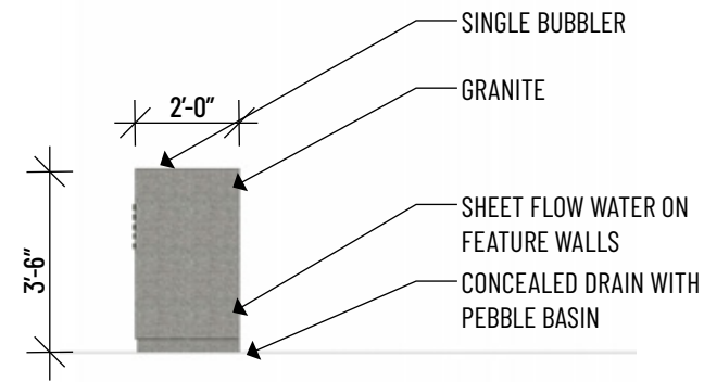
⑤ EAST & WEST ELEVATION (LOWER COURT) 1/4" = 1'-0"
