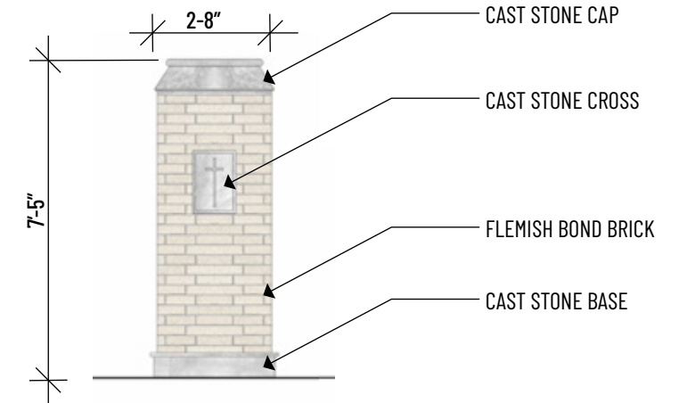
1 NORTH & SOUTH CENTER COLUMBARIUM WALL (UPPER COURT) 1/4" = 1'-0"
