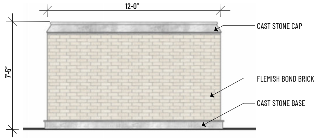
5 WEST SCHOOL COLUMBARIUM WALL (UPPER COURT) 1/4" = 1'-0"
