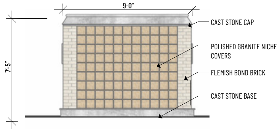
3 EAST CENTER COLUMBARIUM WALL (LOWER COURT) 1/4" = 1'-0"
