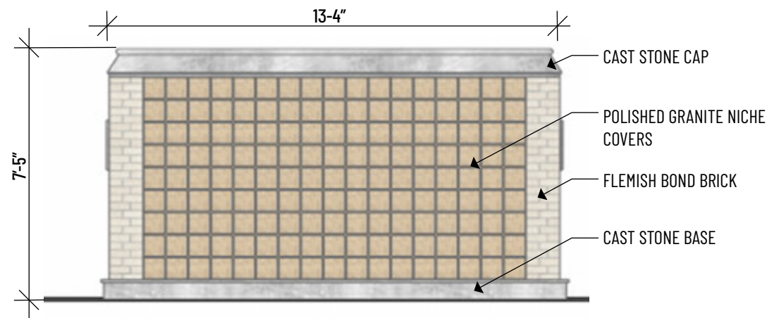
2 EAST CENTER COLUMBARIUM WALL (UPPER COURT) 1/4" = 1'-0"
