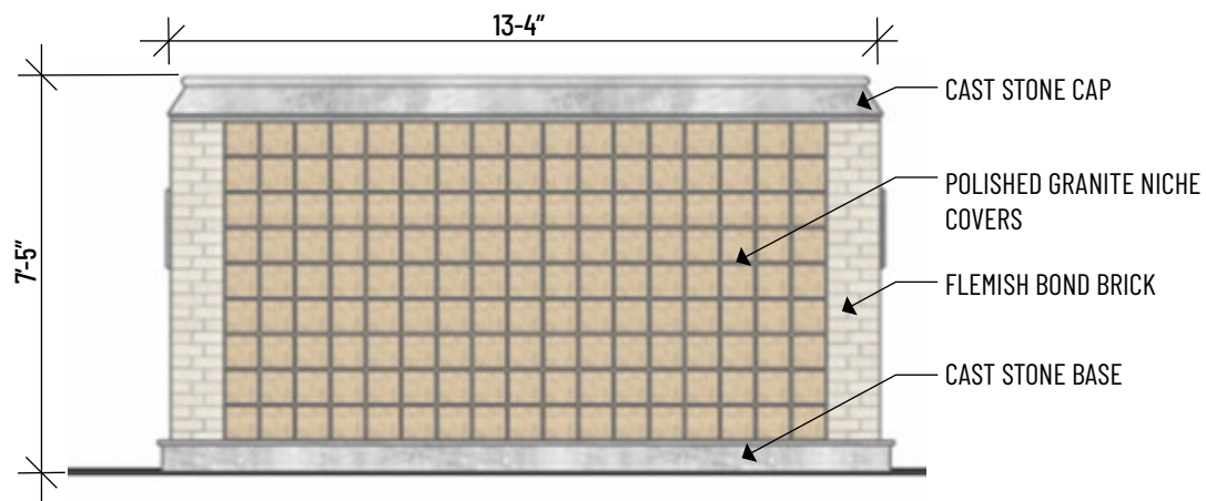
3 WEST CENTER COLUMBARIUM WALL (UPPER COURT) 1/4" = 1'-0"
