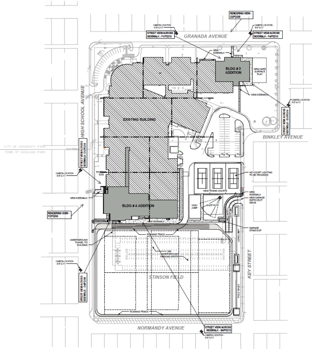
F2 ARCHITECTURAL SITE PLAN F+302
