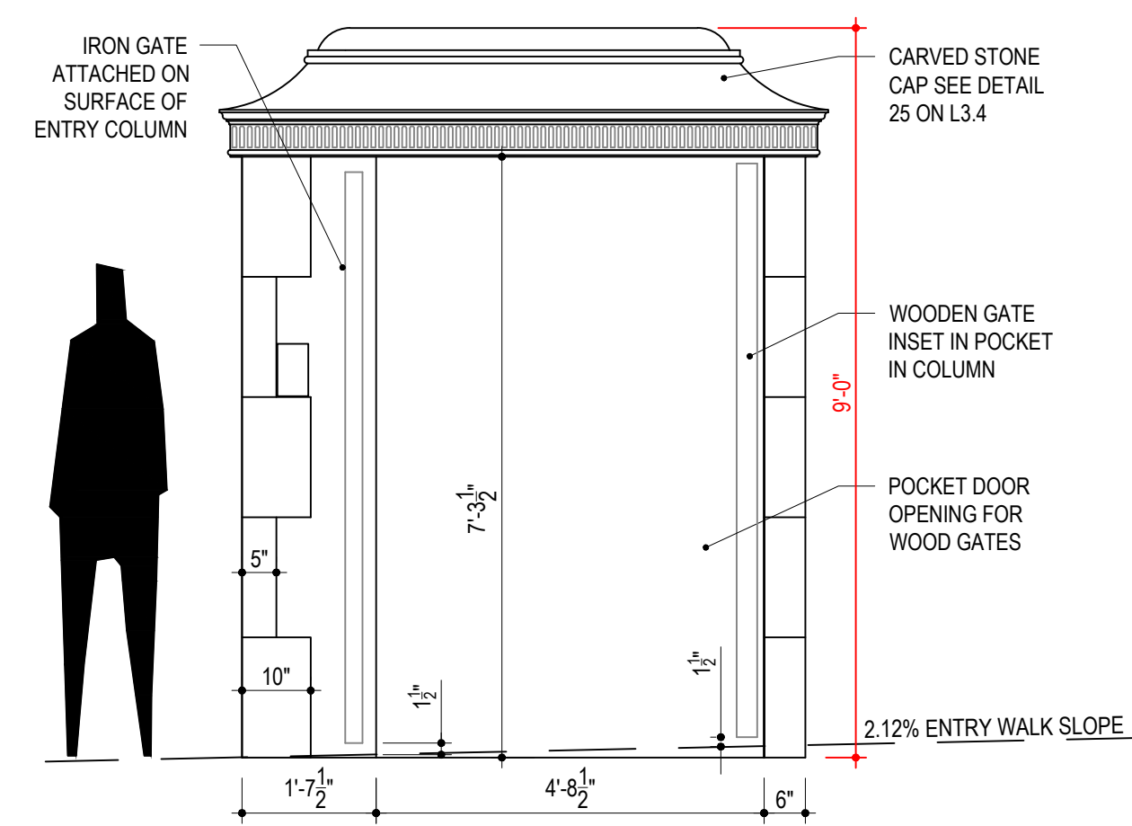
02 FRONT ENTRY COLUMN SCALE: 1/2"=1'-0"
